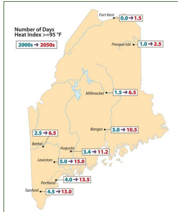
Map 28. Average number of days when the heat index is greater than or equal to 95°F at selected sites for 2000 – 2004 and 2050 – 2054. Predicted values derived from a 48-km downscale simulation of one ensemble member of the CCSM3 model for the IPCC A2 emissions scenario. Source: Fernandez et al. (2015). (Figure from MCC STS. 2020.)
